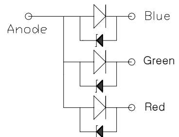
[ INNER CIRCUIT DIAGRAM ]
